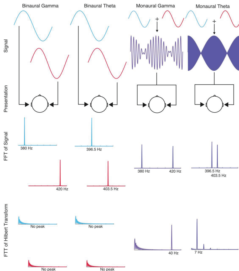
Figure 1. Beats: Signal, Presentation method, Fast Fourier Transform (FFT) and FFT of Hilbert Figure Transform. Each column represents one experimental condition. (Signal and Presentation rows) Binaural beats are created by dichotically presenting two pure tones with a slight frequency mismatch (Red color = right ear). Monaural beats are created by digitally summing these tones and presenting the resulting signal diotically. (FFT of Signal) Stimuli were analyzed using a Fourier transform to obtain their frequency composition. (FFT of Hilbert Transform) The FFT of
